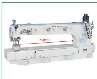
GKP562DL-70 Direct drive long arm post-bed interlock sewing machine with 70cm working space
