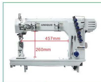
GKP-335-KFD Direct drive walking foot 4-needle 6-thread interlock sewing machine with 457*260mm working space
