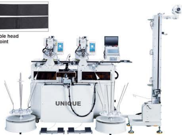
UN-A300P-2-U-VR Full automatic double-station elastic joining machine with auto feeding, ultrasonic cutting and visual recognition Auto over-knotting and length metering Max. elastic width: 7cm Min. elastic circumferences: 20cm
