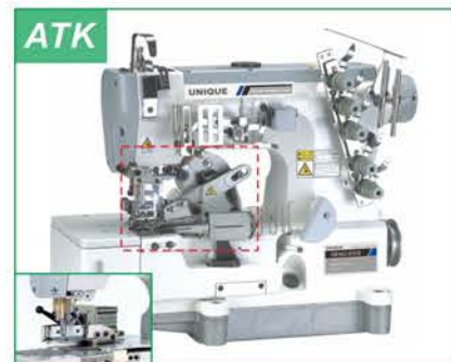
ATK: automatic taper cutter MTK: manual taper cutter GK562-02BB/TK GK562-02BB/TK GK562-04TK GK562-07BB/ATK GK562-02BB/ATK GK562-04/ATK
