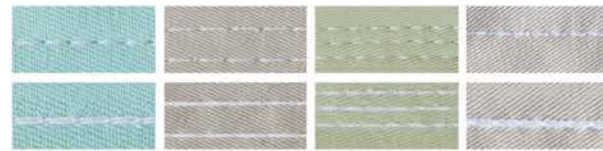
1-needle chainstitch Parallel 2-needle chainstitch 3-needle chainstitch Tandem 2-needle chainstitch
