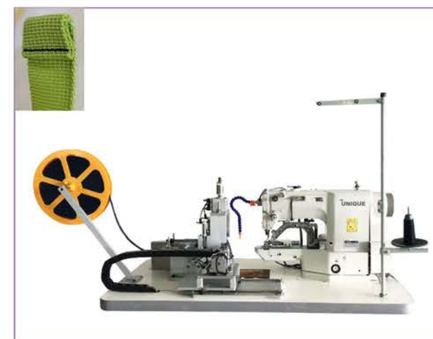
UN430D-ATF-A Full automatic ribbon belt folding and bartacking machine with auto tape feeding and cutting
