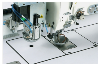
Knife cutting function
