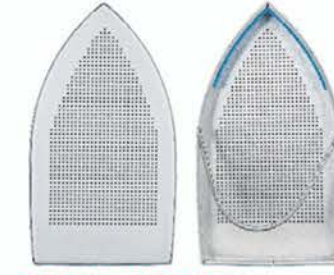
TIS-A/SHELDON-555 50 220×121mm
